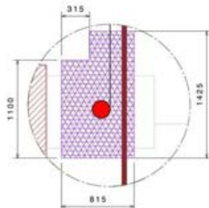
Detail A Scale : 1:25
