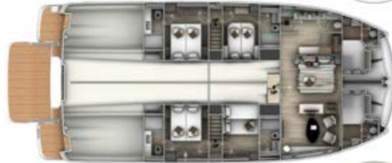
Galley up layout 5 staterooms, 5 bathrooms, 2 crew cabins
