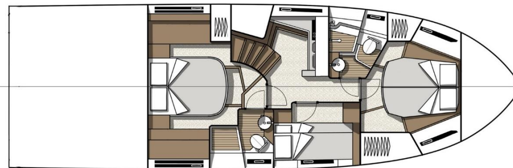
3 cabin version
